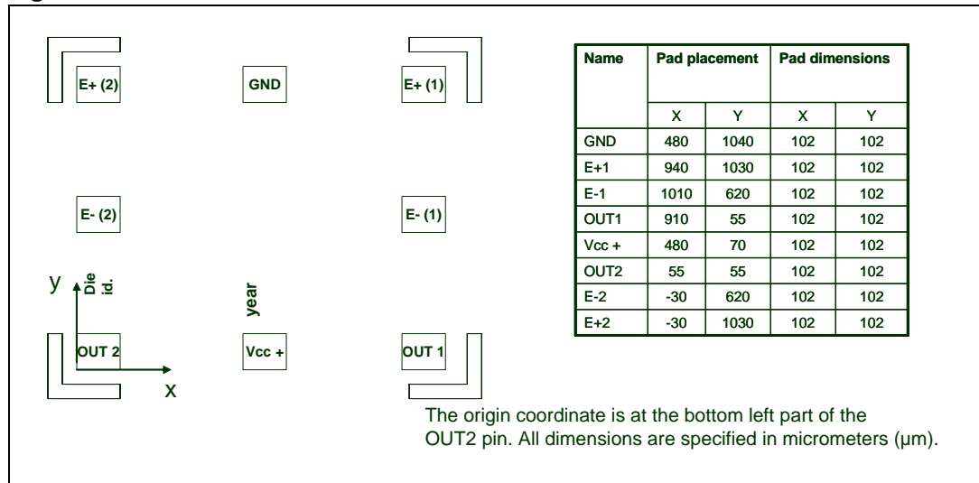
Figure 2. Pad locations
